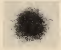
Strain AS
